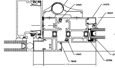
7B 112-7B OPTIONAL IS HINGE JAMB SSG
