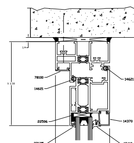
5C 112-5C OPTIONAL IS HEAD
