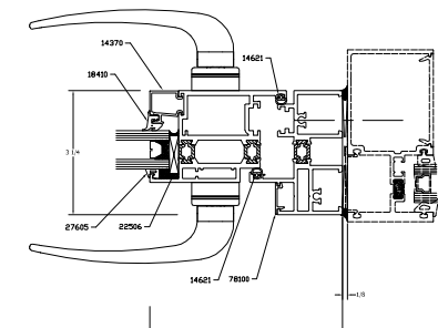
8 112-8 STANDARD IS LOCK JAMB FLAT
