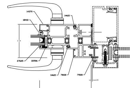
8A 112-8A OPTIONAL IS LOCK JAMB CAPTURED
