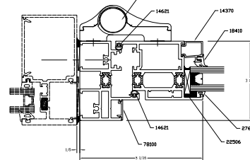
7 112-7 STANDARD IS HINGE JAMB FLAT
