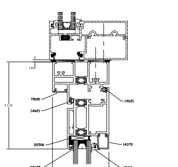
5 112-5 STANDARD IS HEAD FLAT
