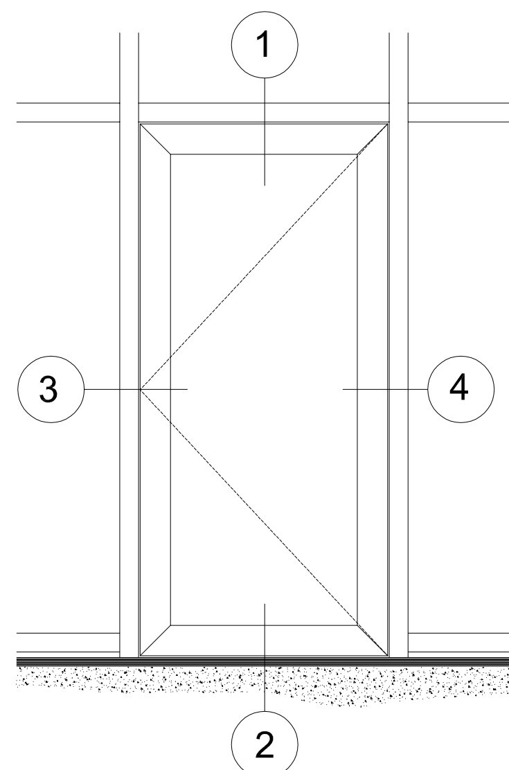
OUTSWING ELEVATION
