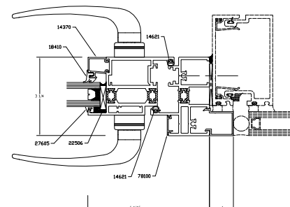
8B 112-8B OPTIONAL IS LOCK JAMB SSG
