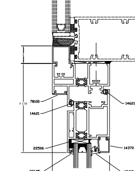
5B 112-5B OPTIONAL IS HEAD SSG
