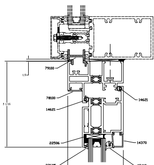
5A 112-5A OPTIONAL IS HEAD CAPTURED
