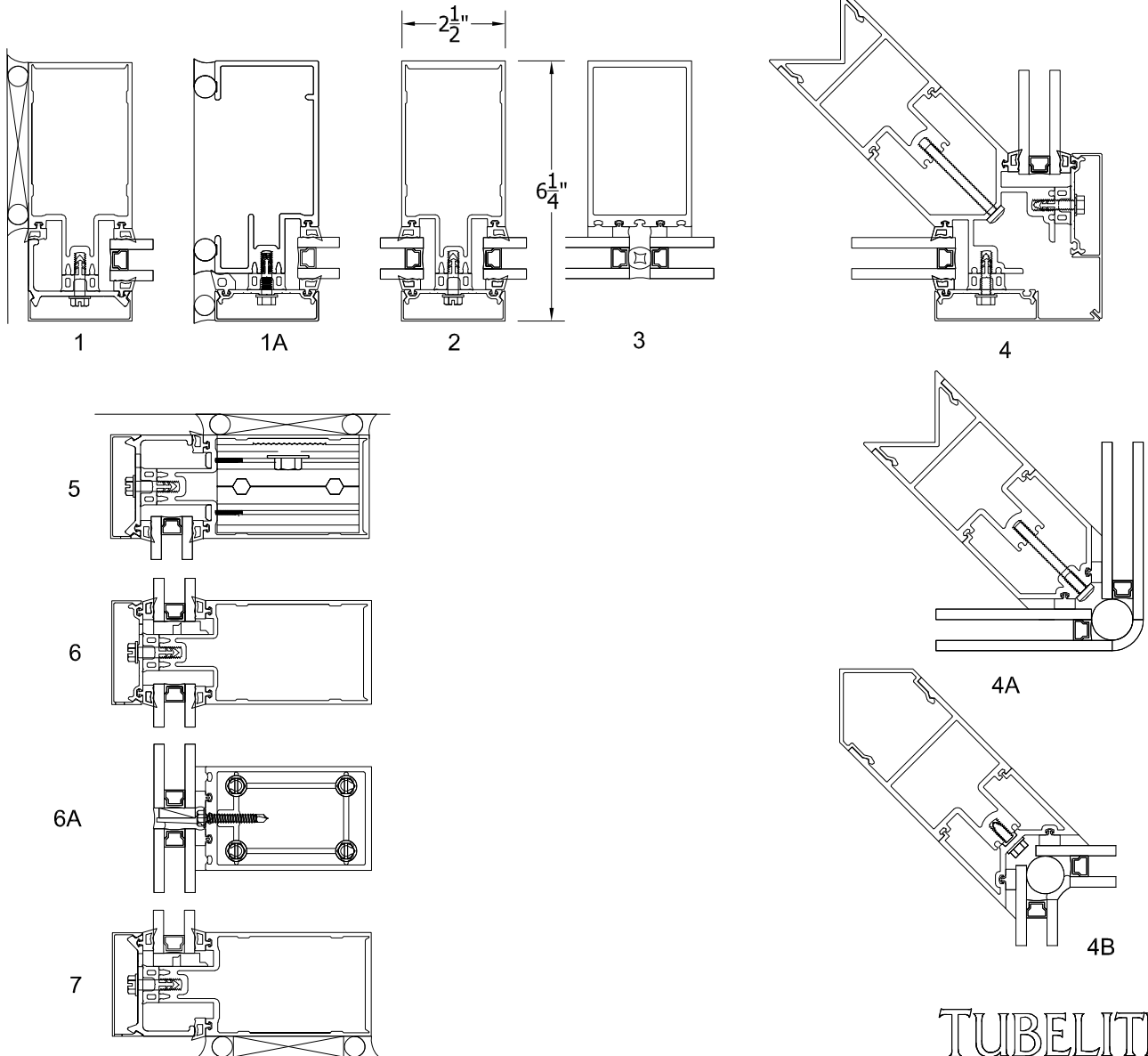
400T Series Curtain Wall also available with thermal pressure plates
