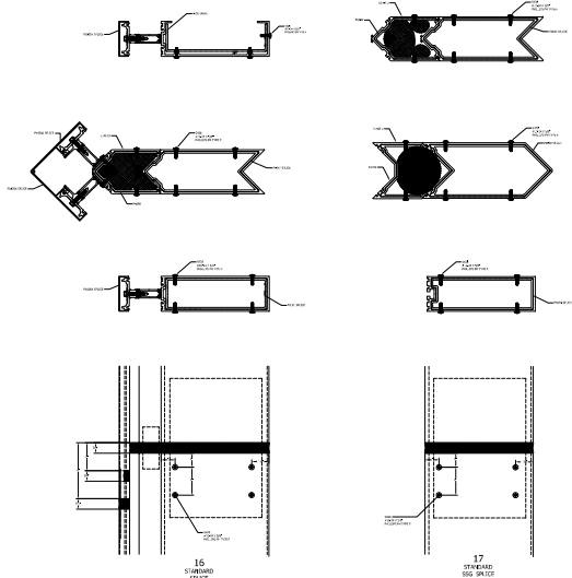
SPLICE AND ANCHOR DETAILS
