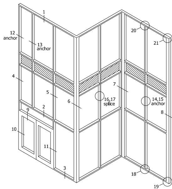
TYPICAL ELEVATION
