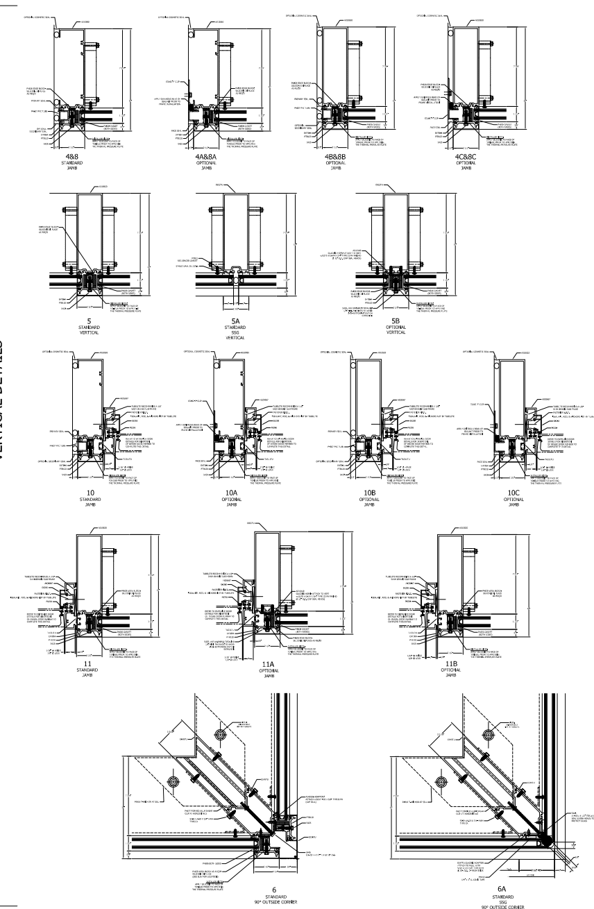
VERTICAL DETAILS
