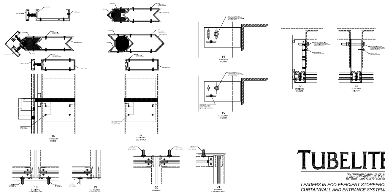
SPLICE AND ANCHOR DETAILS
