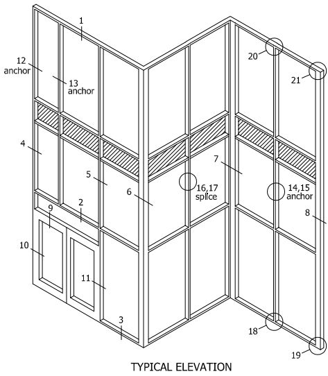
TYPICAL ELEVATION
