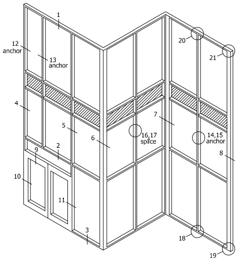
TYPICAL ELEVATION
