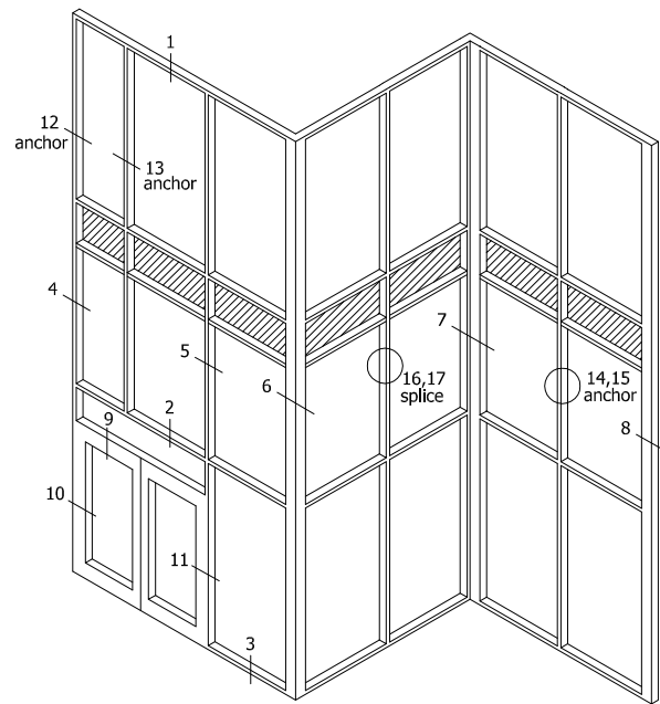
TYPICAL ELEVATION
