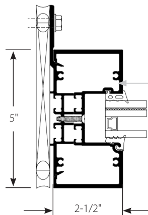
Screw Spline Frame Construction
