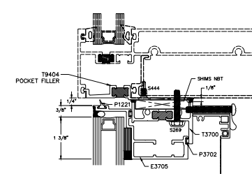
21 HEAD FLATBACK INSTALLATION STANDARD
