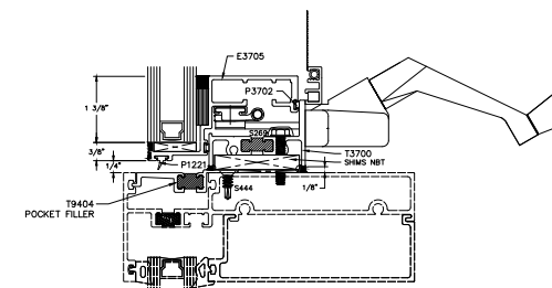
22 SILL FLATBACK INSTALLATION STANDARD
