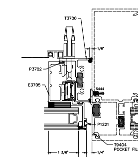
24 JAMB FLATBACK INSTALLATION STANDARD
