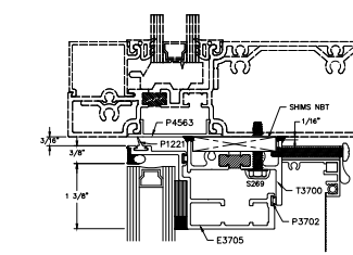
17B HEAD SF ADAPTER OPTIONAL
