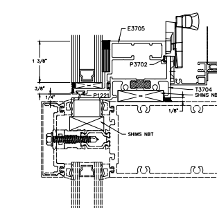
18A SILL GLAZED-IN FRAME OPTIONAL
