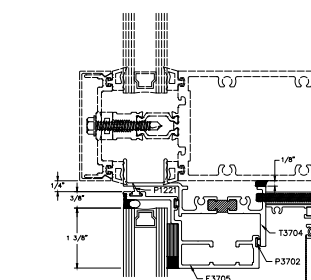
21A HEAD GLAZED-IN FRAME OPTIONAL
