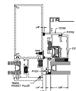
19 JAMB FLATBACK INSTALLATION STANDARD
