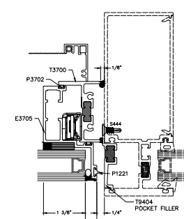
20 JAMB FLATBACK INSTALLATION STANDARD
