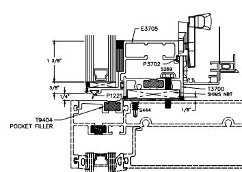
18 SILL FLATBACK INSTALLATION STANDARD
