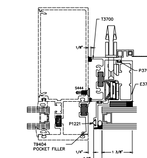
23 JAMB FLATBACK INSTALLATION STANDARD
