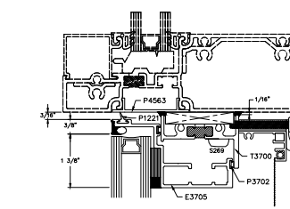
21B HEAD SF ADAPTER OPTIONAL
