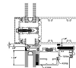
17A HEAD GLAZED-IN FRAME OPTIONAL
