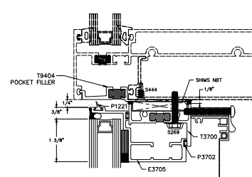
17 HEAD FLATBACK INSTALLATION STANDARD
