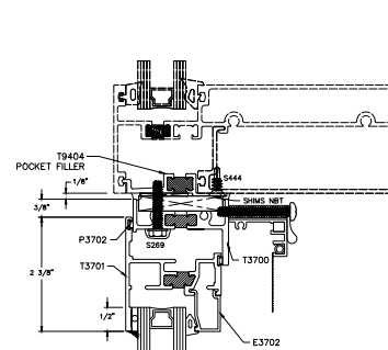
9 HEAD FLATBACK INSTALLATION STANDARD
