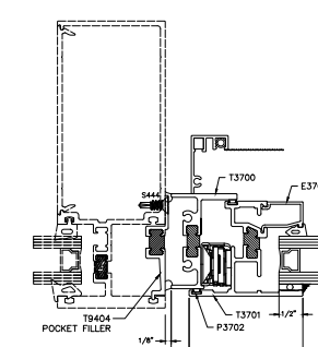
11 JAMB FLATBACK INSTALLATION STANDARD
