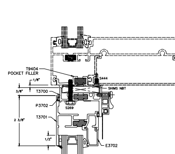
13 HEAD FLATBACK INSTALLATION STANDARD
