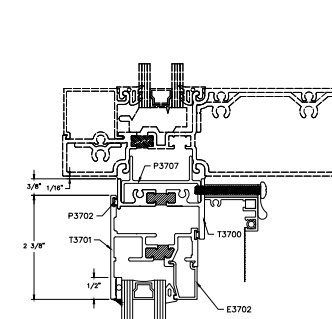
9B HEAD SF ADAPTER OPTIONAL
