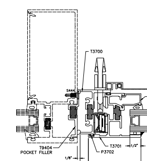
15 JAMB FLATBACK INSTALLATION STANDARD
