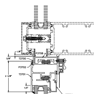
13A HEAD CW ADAPTER OPTIONAL
