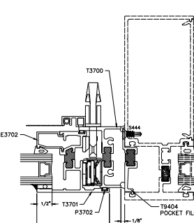
16 JAMB FLATBACK INSTALLATION STANDARD
