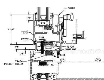
10 SILL FLATBACK INSTALLATION STANDARD
