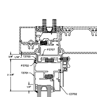
13B HEAD SF ADAPTER OPTIONAL
