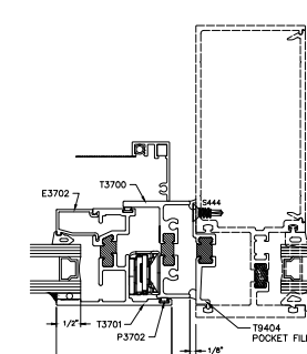
12 JAMB FLATBACK INSTALLATION STANDARD
