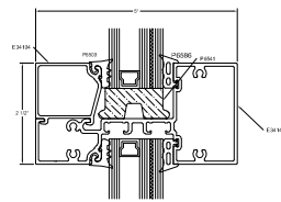
DRY GLAZE DETAIL
