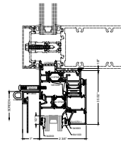
1A HEAD CURTAIN WALL INSTALLATION OPTIONAL
