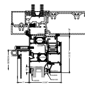
1B HEAD SF ADAPTOR INSTALLATION OPTIONAL
