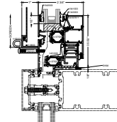
2A SILL CURTAIN WALL INSTALLATION OPTIONAL
