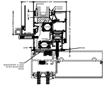
2 SILL FLATBACK INSTALLATION STANDARD
