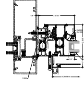
3B SF INSTALLATION OPTIONAL
