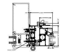
7 FLATBACK INSTALLATION STANDARD
