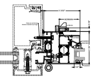
7A CURTAIN WALL INSTALLATION OPTIONAL
