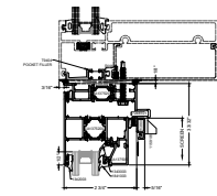
5 HEAD FLATBACK INSTALLATION STANDARD
