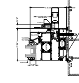
8B JAMB SF INSTALLATION OPTIONAL
