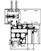
1A HEAD CURTAIN WALL INSTALLATION OPTIONAL
