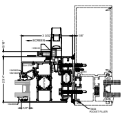
8 JAMB FLATBACK INSTALLATION STANDARD
