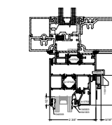
5B HEAD SF ADAPTOR OPTIONAL
