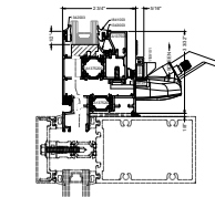
6A SILL CURTAIN WALL INSTALLATION OPTIONAL
