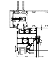
5A HEAD CURTAIN WALL INSTALLATION OPTIONAL
