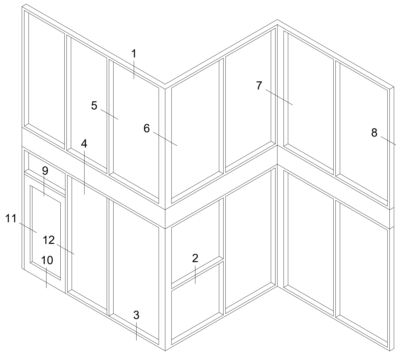
TYPICAL ELEVATION
