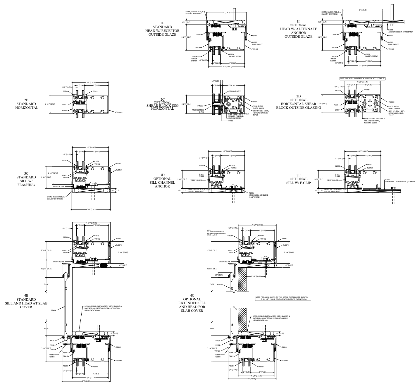
OUTSIDE GLAZED HORIZONTAL DETAILS
