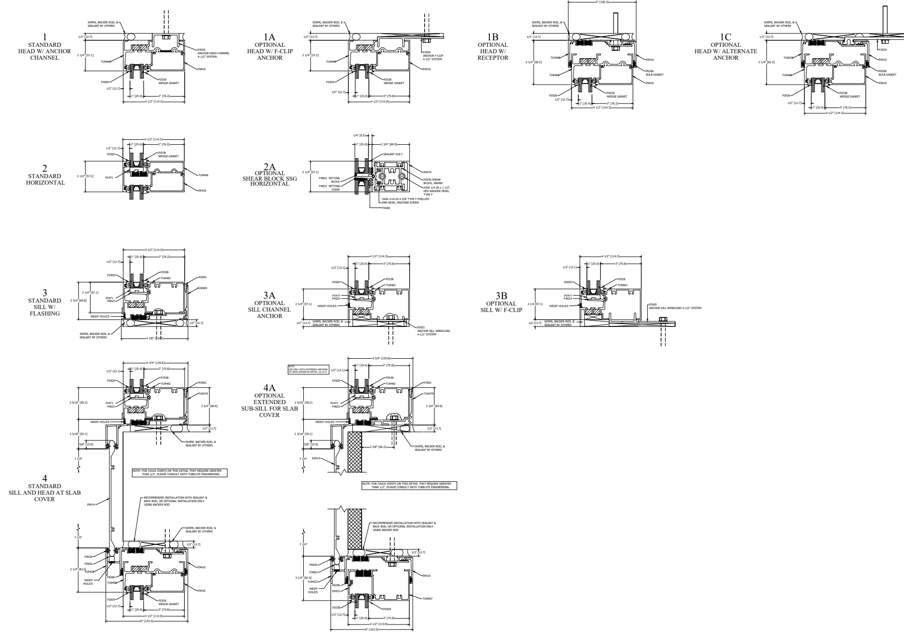
INSIDE GLAZED HORIZONTAL DETAILS
