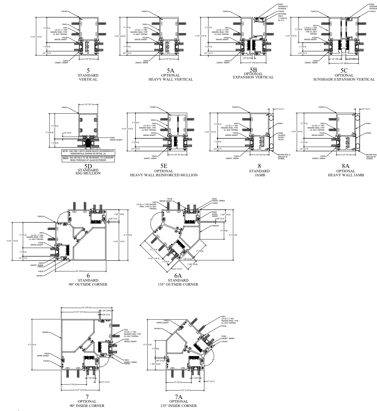
INSIDE GLAZED VERTICAL DETAILS
