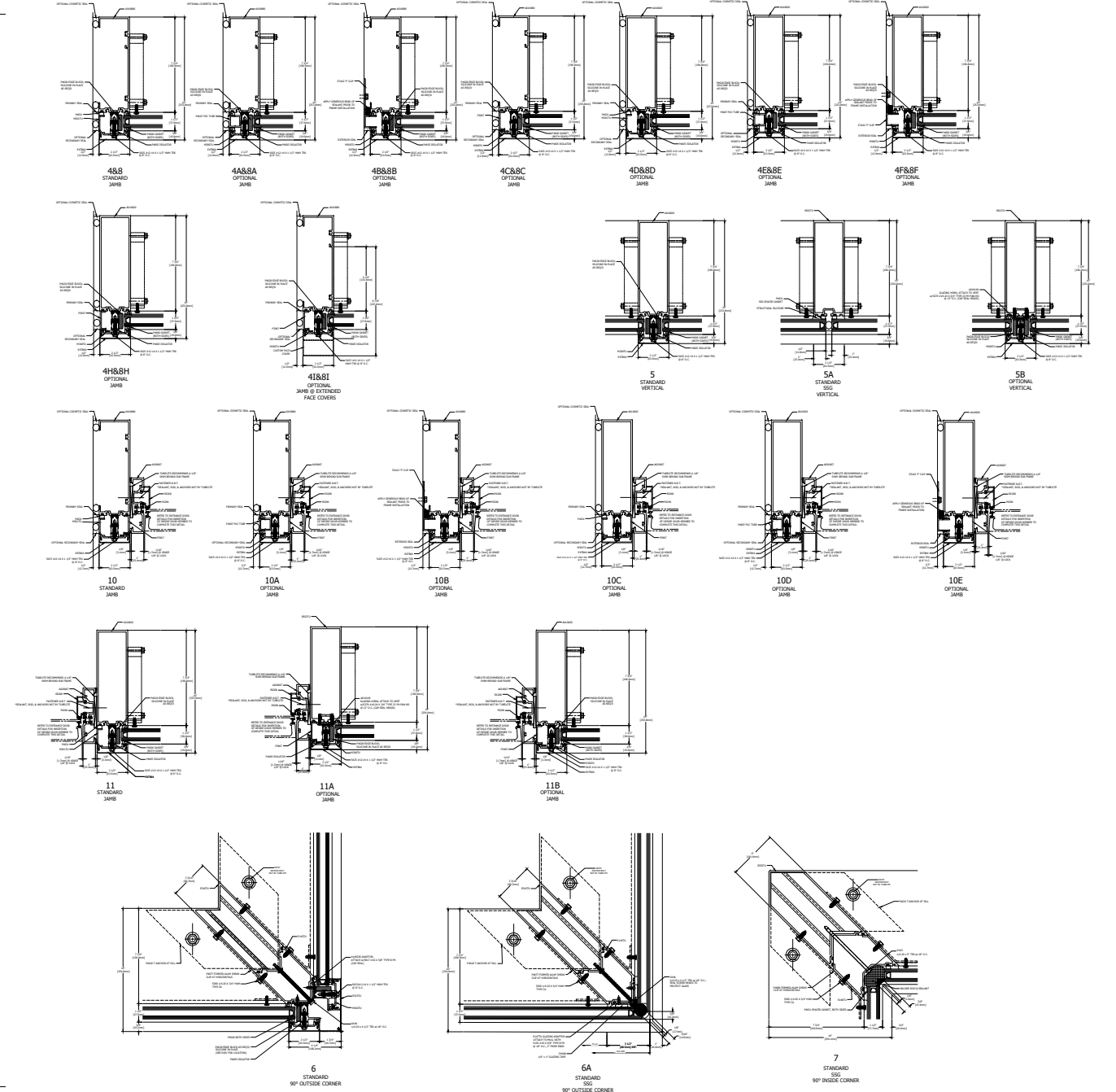
VERTICAL DETAILS
