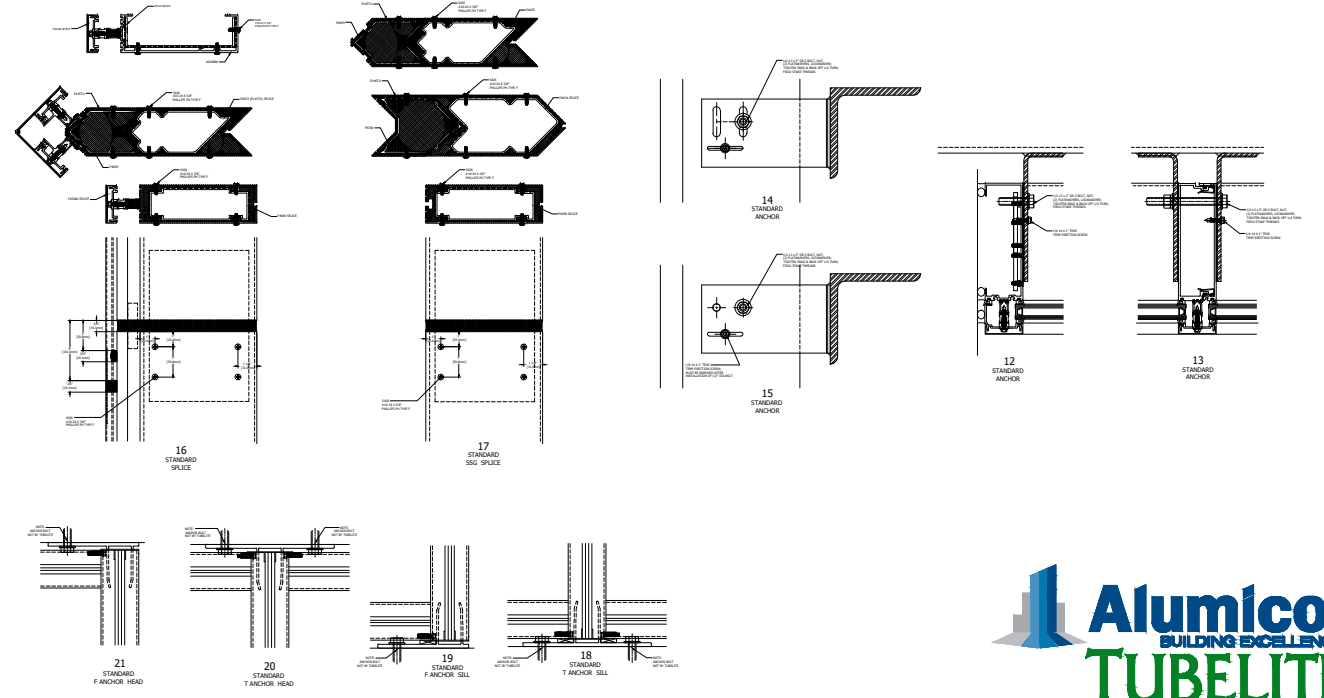
SPLICE AND ANCHOR DETAILS
