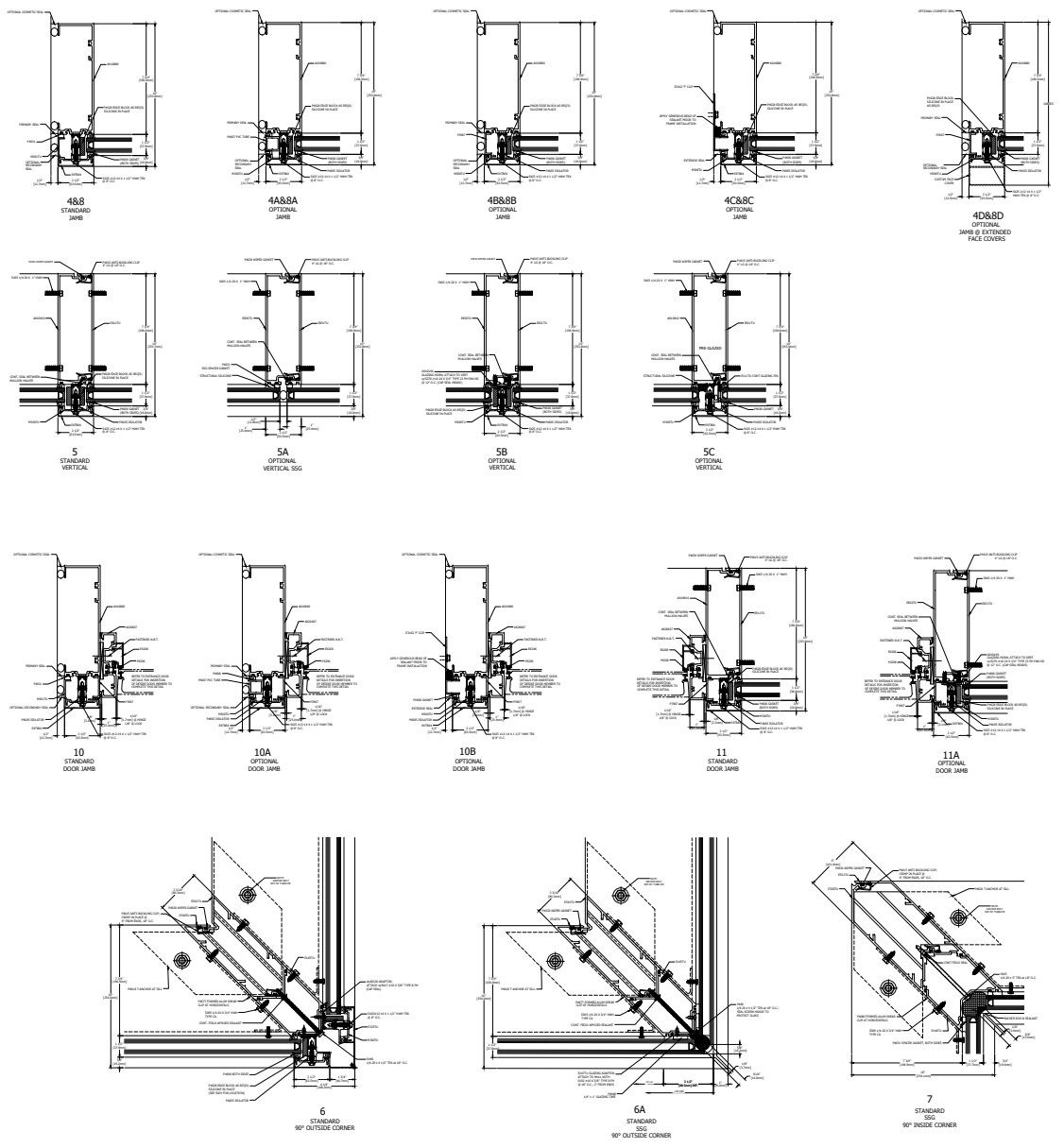
VERTICAL DETAILS
