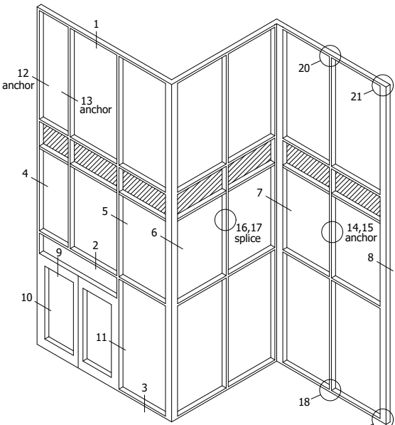
TYPICAL ELEVATION
