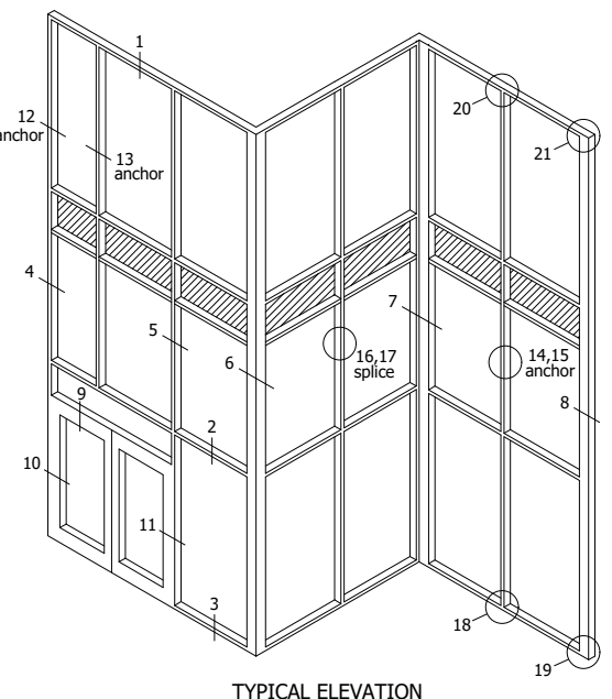
TYPICAL ELEVATION
