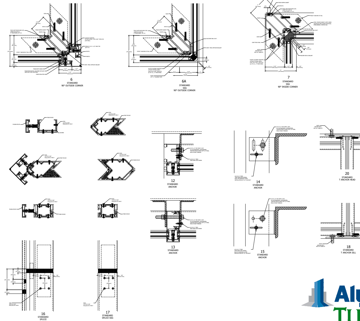
SPLICE AND ANCHOR DETAILS
