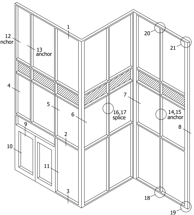
TYPICAL ELEVATION
