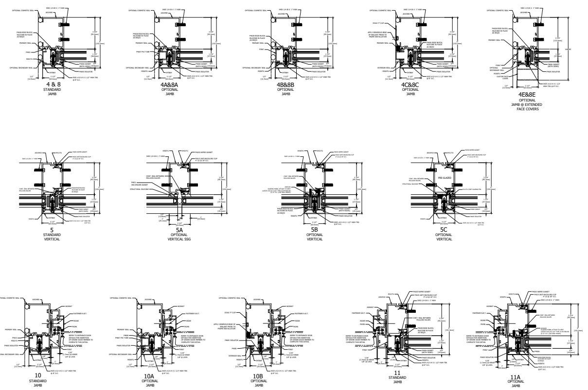
VERTICAL DETAILS
