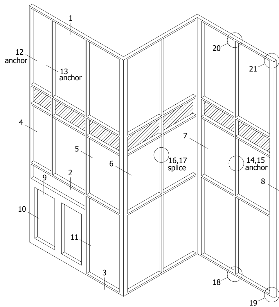
TYPICAL ELEVATION
