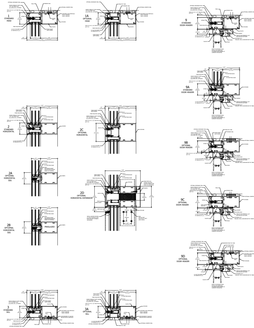
VERTICAL DETAILS
