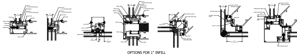
HORIZONTAL DETAILS
