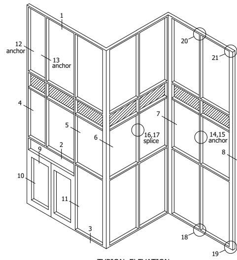
TYPICAL ELEVATION
