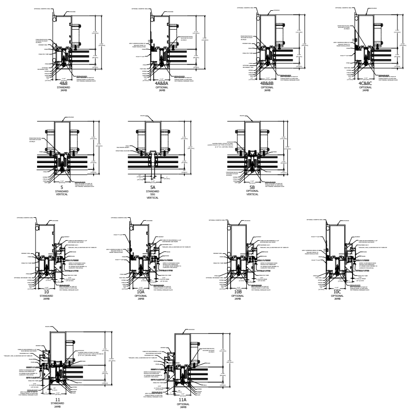
VERTICAL DETAILS
