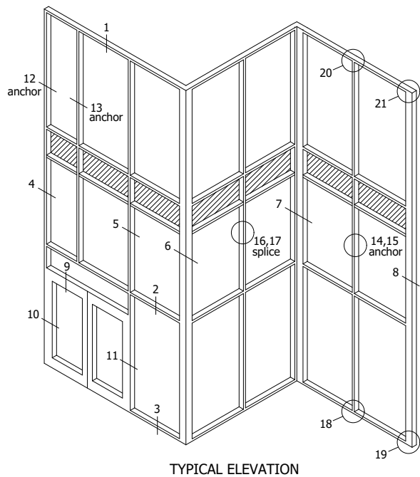
TYPICAL ELEVATION
