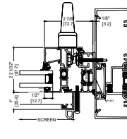
4B JAMB SF INSTALLATION STANDARD
