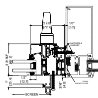
4 JAMB FLATBACK INSTALLATION STANDARD
