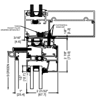
1 HEAD FLATBACK INSTALLATION STANDARD
