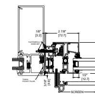
3 FLATBACK INSTALLATION STANDARD
