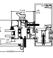
4A JAMB CURTAIN WALL INSTALLATION STANDARD
