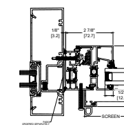
3B SF INSTALLATION STANDARD
