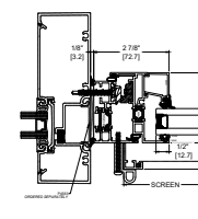
3B SF INSTALLATION STANDARD
