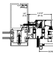
3A CURTAIN WALL INSTALLATION STANDARD
