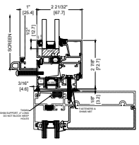
2 SILL FLATBACK INSTALLATION STANDARD
