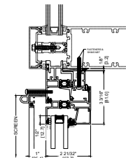
1A HEAD CURTAIN WALL INSTALLATION STANDARD
