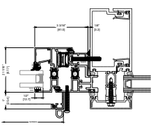
4A JAMB CURTAIN WALL INSTALLATION STANDARD
