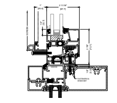
2B SILL SF ADAPTOR STANDARD
