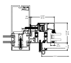
3A CURTAIN WALL INSTALLATION STANDARD
