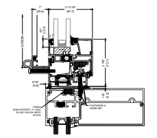
2 SILL FLATBACK INSTALLATION STANDARD
