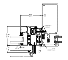
4 JAMB FLATBACK INSTALLATION STANDARD
