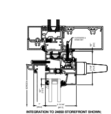
1B HEAD SF ADAPTOR STANDARD
