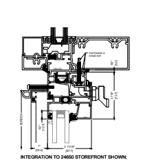
1B HEAD SF ADAPTOR STANDARD
