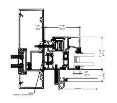
3B SF INSTALLATION STANDARD
