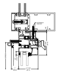
1A HEAD CURTAIN WALL INSTALLATION STANDARD
