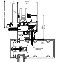
2A SILL CURTAIN WALL INSTALLATION STANDARD
