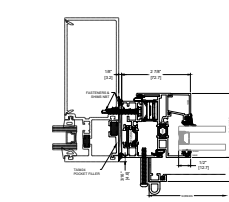
3 FLATBACK INSTALLATION STANDARD
