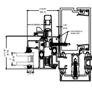
8A JAMB CURTAIN WALL INSTALLATION STANDARD
