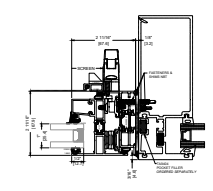
8 JAMB FLATBACK INSTALLATION STANDARD
