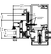
4A JAMB CURTAIN WALL INSTALLATION STANDARD
