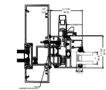
7B FLATBACK SF INSTALLATION STANDARD
