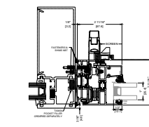
7 FLATBACK INSTALLATION STANDARD
