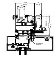
2B SILL SF ADAPTOR STANDARD
