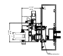
8B JAMB SF INSTALLATION STANDARD
