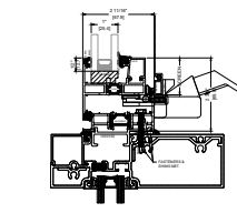
6B SILL SF ADAPTOR STANDARD
