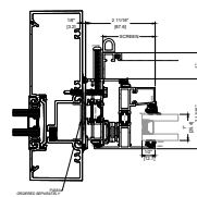
3B FLATBACK SF INSTALLATION STANDARD
