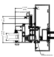
4B JAMB SF INSTALLATION STANDARD
