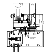
2A SILL CURTAIN WALL INSTALLATION STANDARD
