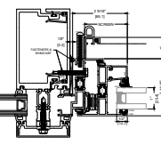
3A FLATBACK CURTAIN WALL INSTALLATION STANDARD
