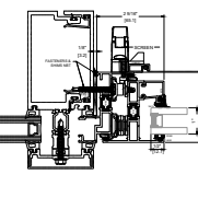
7A FLATBACK CURTAIN WALL INSTALLATION STANDARD
