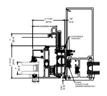
4 JAMB FLATBACK INSTALLATION STANDARD
