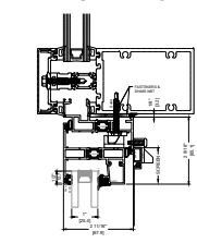
5A HEAD CURTAIN WALL INSTALLATION STANDARD
