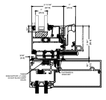
2 SILL FLATBACK INSTALLATION STANDARD
