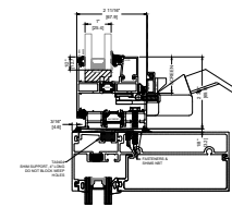
6 SILL FLATBACK INSTALLATION STANDARD
