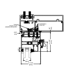
5 HEAD FLATBACK INSTALLATION STANDARD
