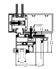
1A HEAD CURTAIN WALL INSTALLATION STANDARD
