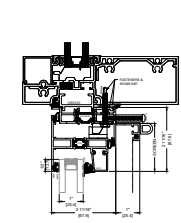
1B HEAD SF ADAPTOR STANDARD
