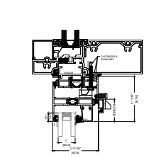
5B HEAD SF ADAPTOR STANDARD
