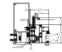
3 FLATBACK INSTALLATION STANDARD
