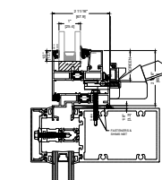
6A SILL CURTAIN WALL INSTALLATION STANDARD
