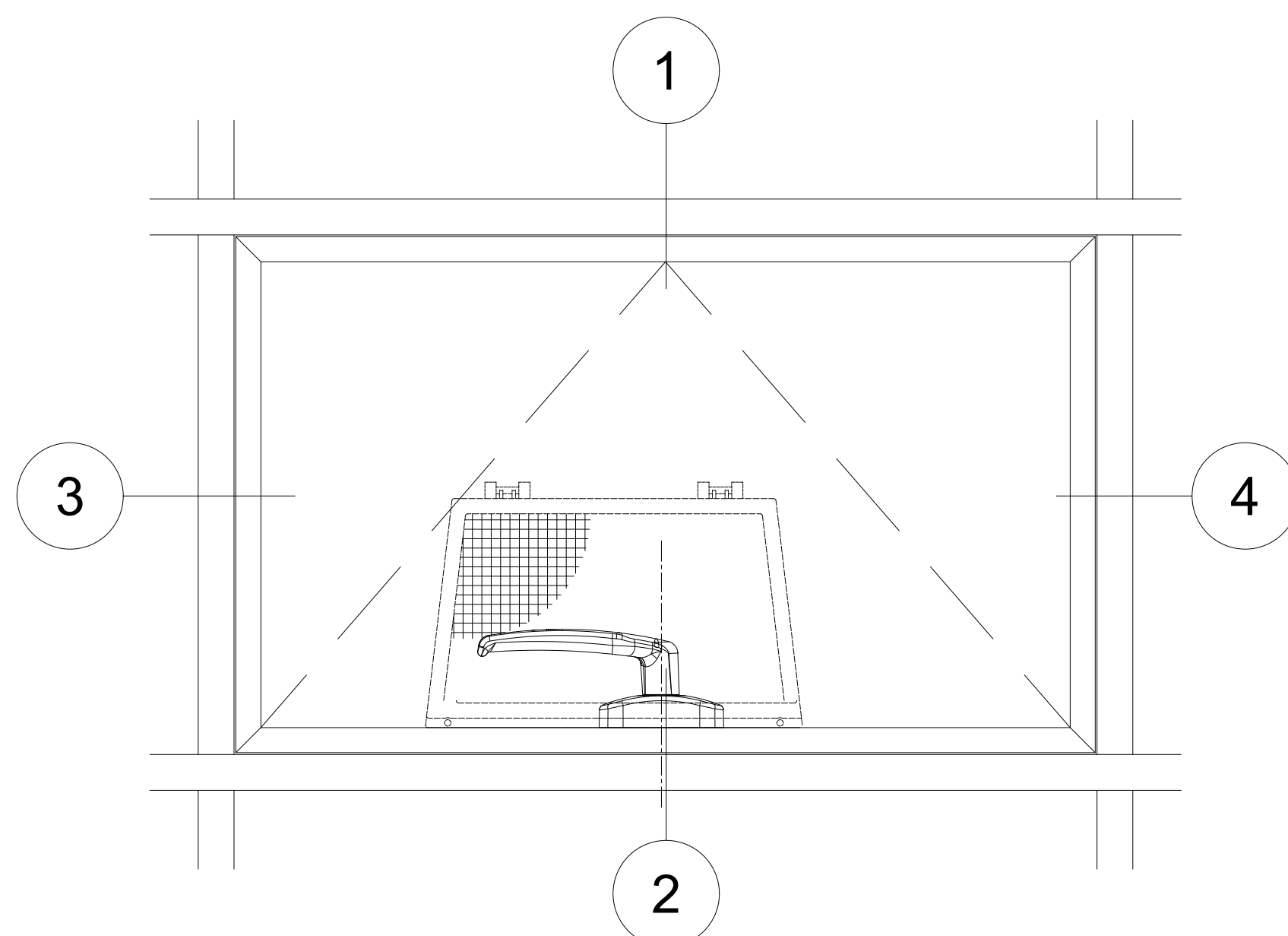
TYPICAL ELEVATION 4-BAR / MPL HANDLE WITH OPTIONAL SCREEN
