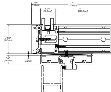
HORIZONTAL DETAILS
