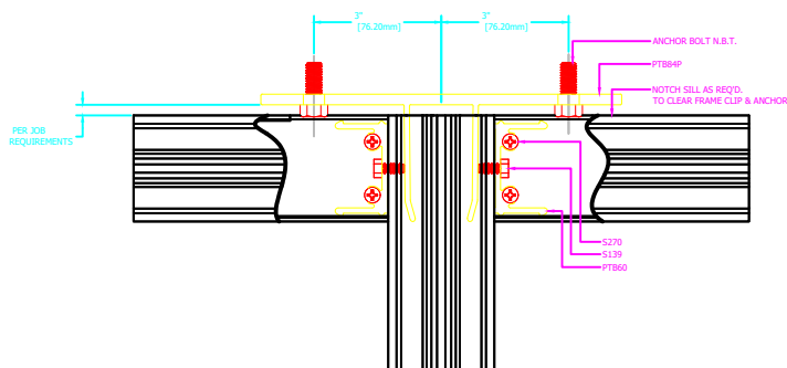
TYPICAL ELEVATION
