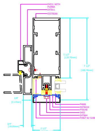
8 STANDARD DOOR JAMB AT SIDELITE W/ VINYL POCKET CLOSER
