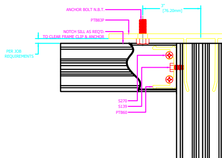
13 STANDARD "F" ANCHOR AT HEAD
