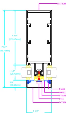
6 STANDARD TUBULAR MULLION
