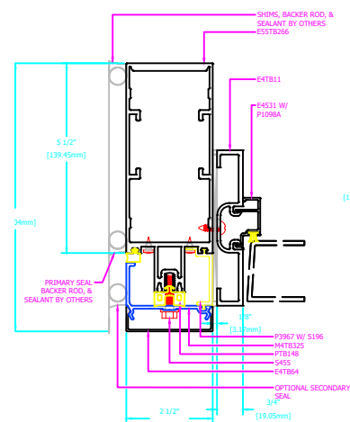
7 STANDARD DOOR JAMB AT PERIMETER PRESSURE PLATE W/ ALUMINUM POCKET CLOSER
