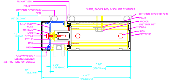
1 STANDARD HEAD
