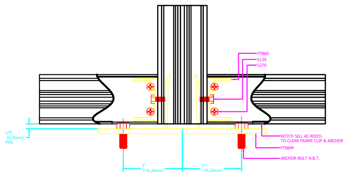
14 STANDARD "T" ANCHOR AT SILL
