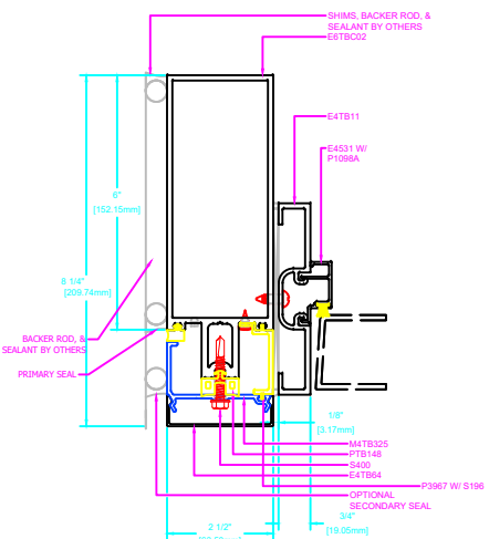
7 STANDARD DOOR JAMB AT PERIMETER PRESSURE PLATE W/ ALUMINUM POCKET CLOSER
