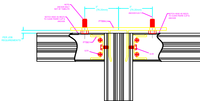
TYPICAL ELEVATION
