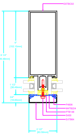
6 STANDARD TUBULAR MULLION
