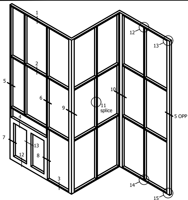
TYPICAL ELEVATION
