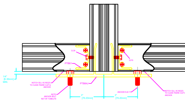
14 STANDARD "T" ANCHOR AT SILL
