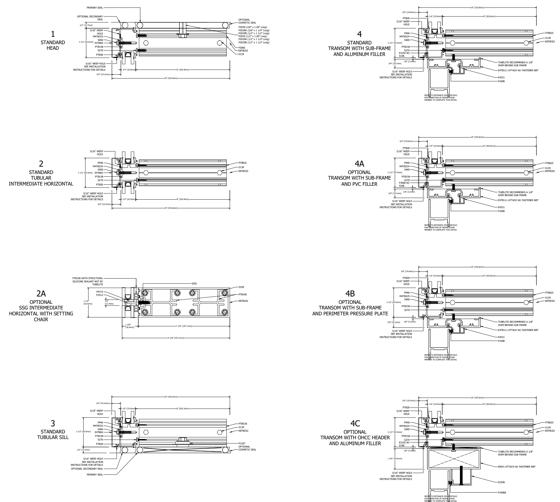
HORIZONTAL DETAILS
