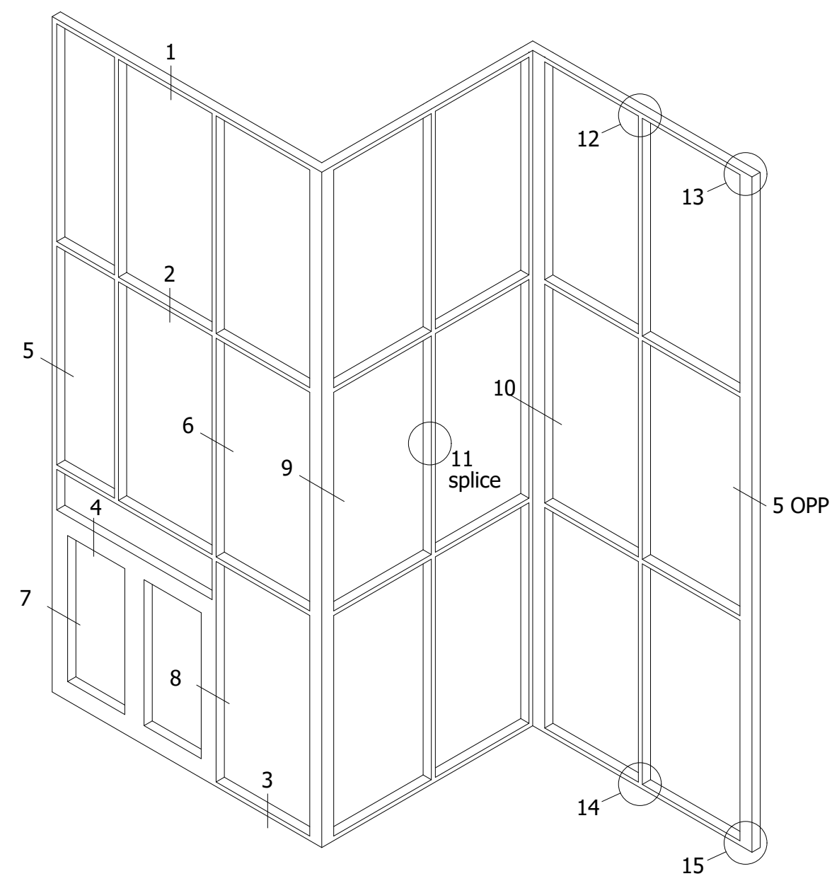
TYPICAL ELEVATION
