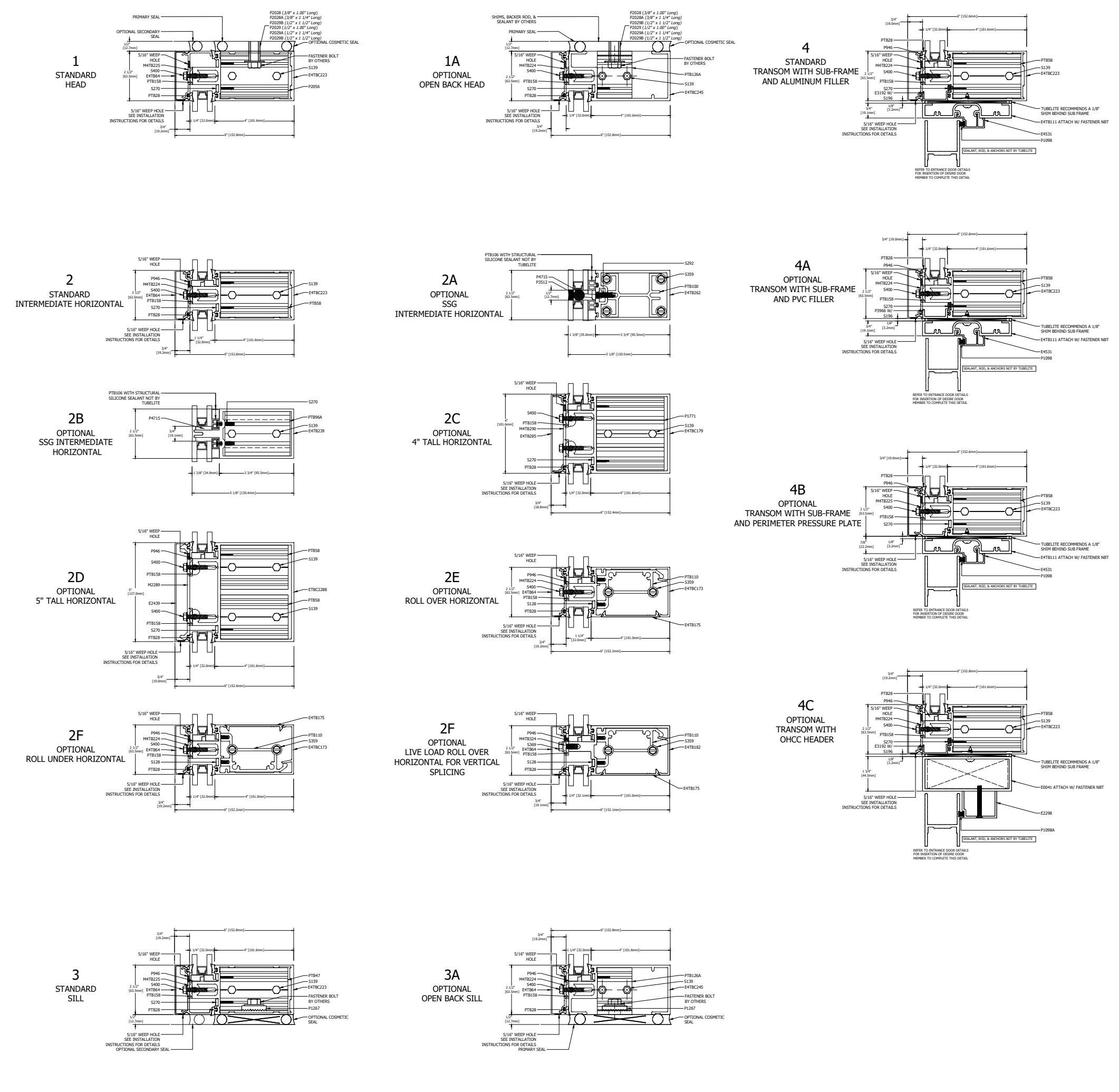
HORIZONTAL DETAILS
