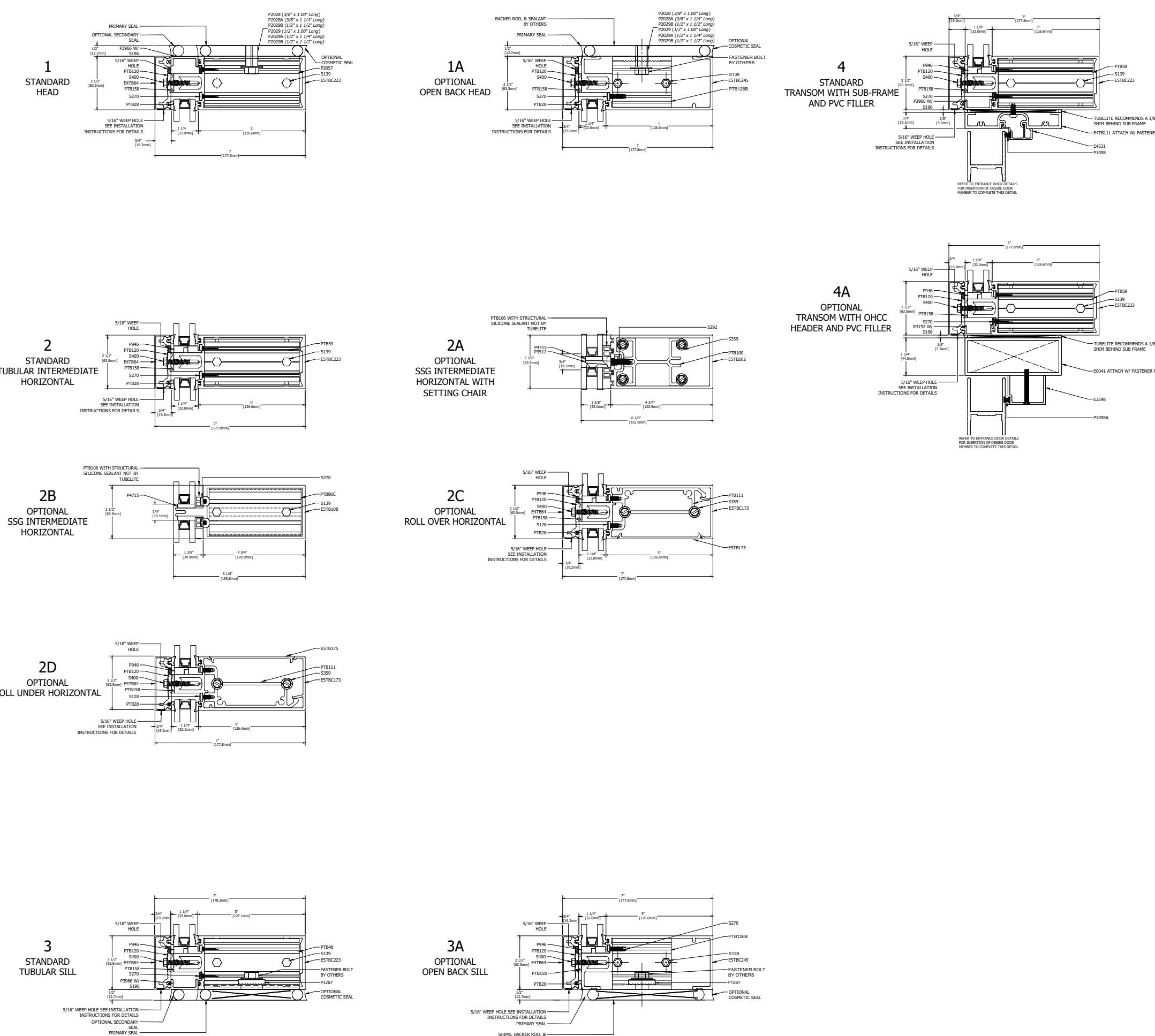
HORIZONTAL DETAILS
