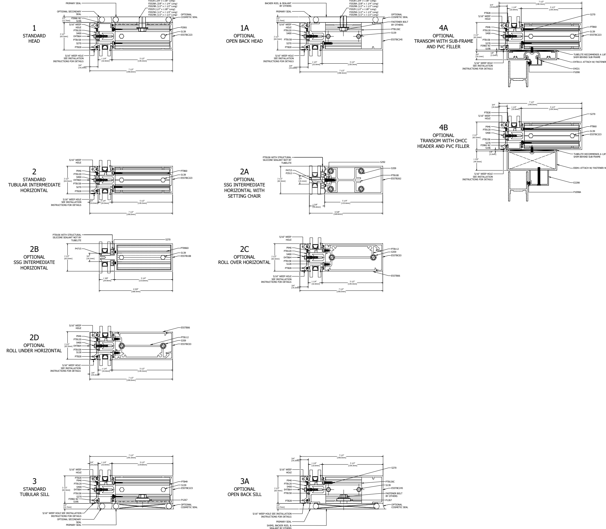
VERTICAL DETAILS
