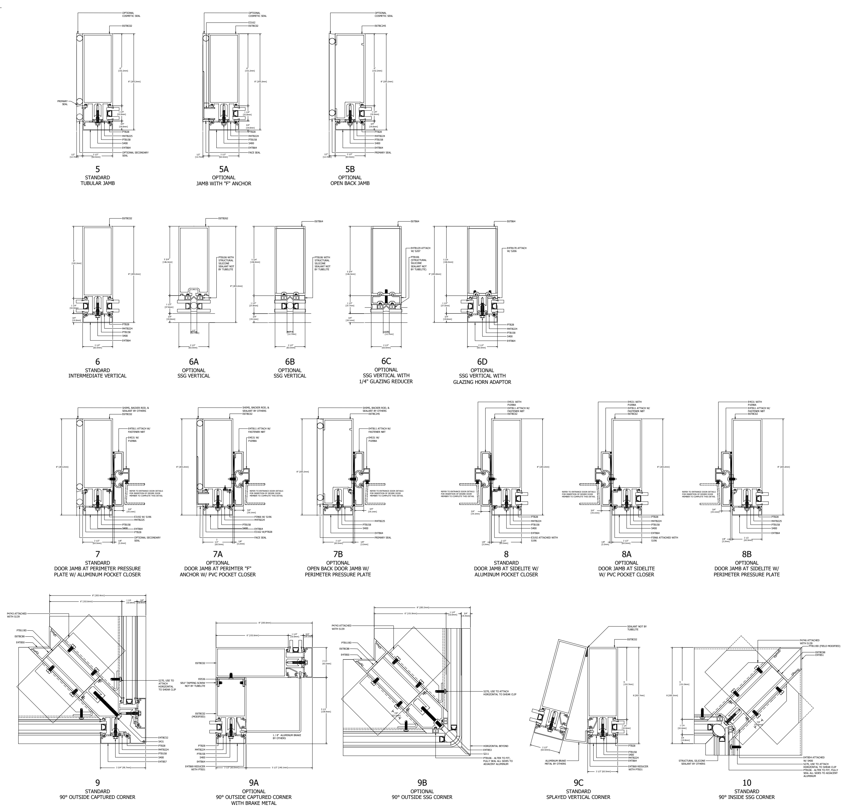
VERTICAL DETAILS
