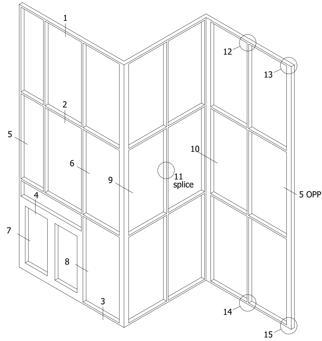
TYPICAL ELEVATION
