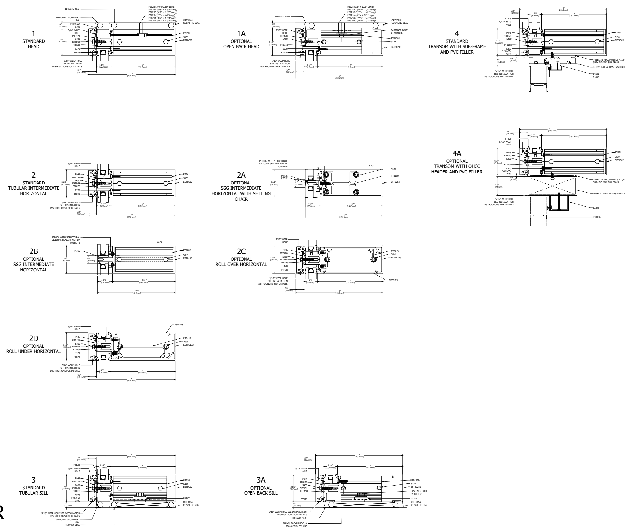
HORIZONTAL DETAILS
