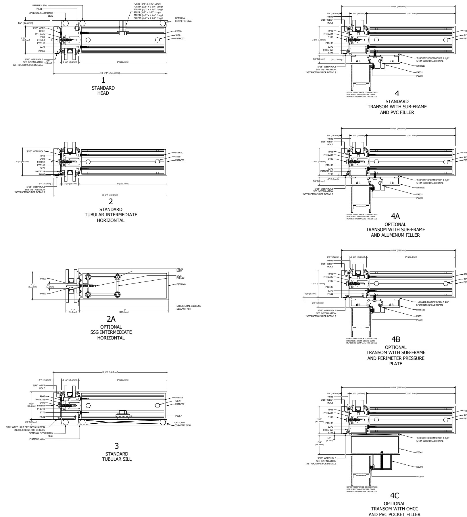
HORIZONTAL DETAILS
