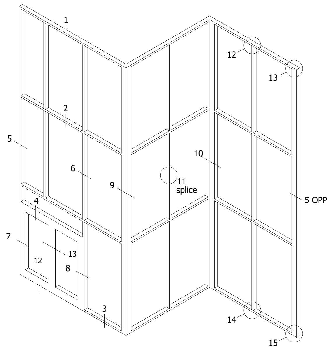
TYPICAL ELEVATION 400T SERIES
