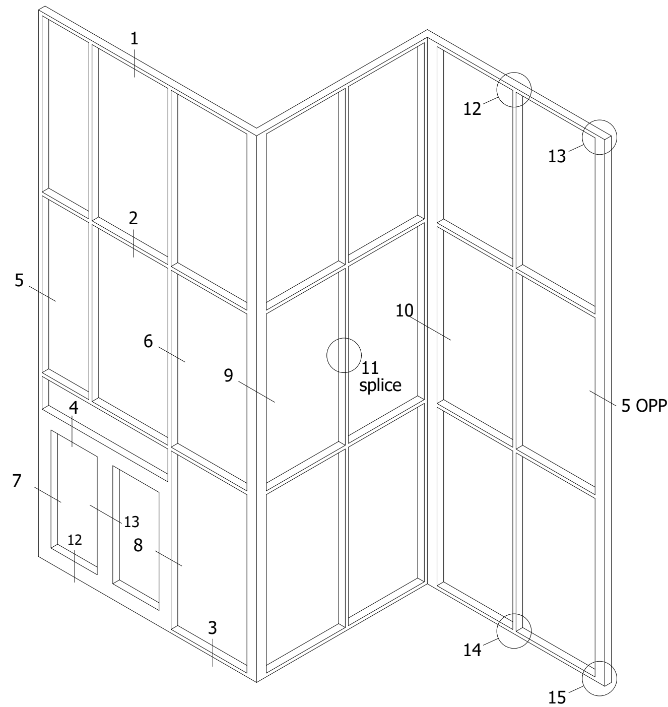
TYPICAL ELEVATION
