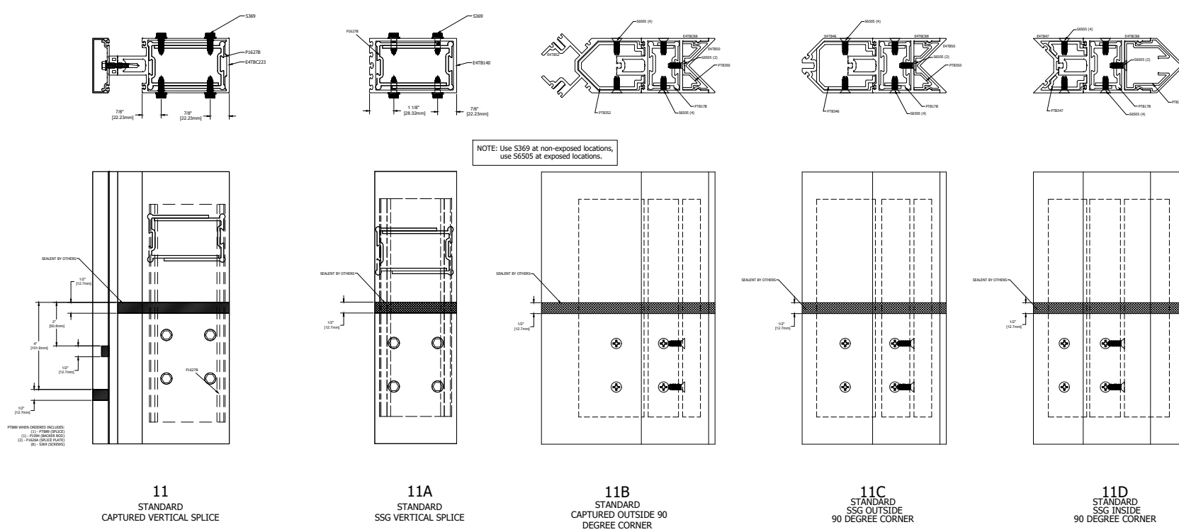
SPLICE AND ANCHOR DETAILS
