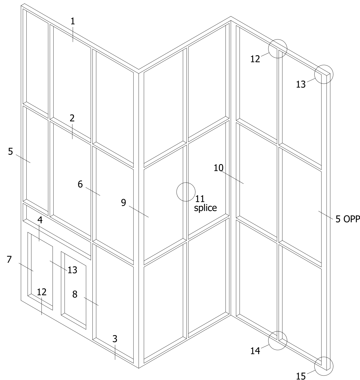
TYPICAL ELEVATION
