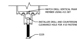
SCREW APPLIED HORN
