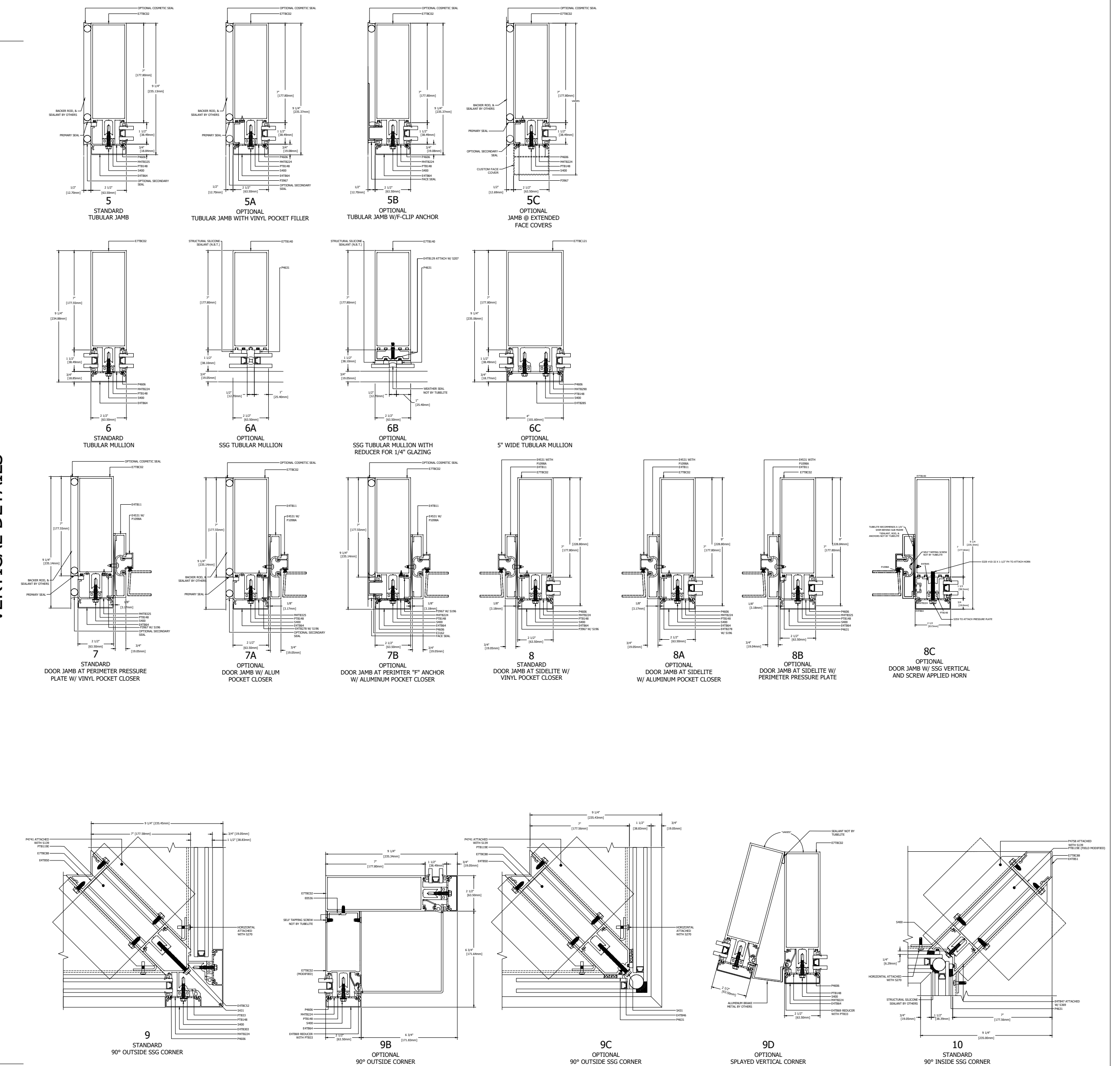
VERTICAL DETAILS
