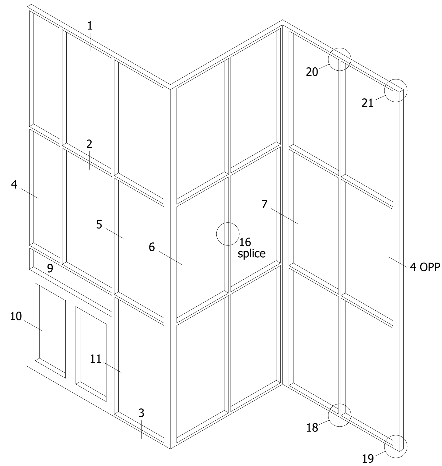
TYPICAL ELEVATION
