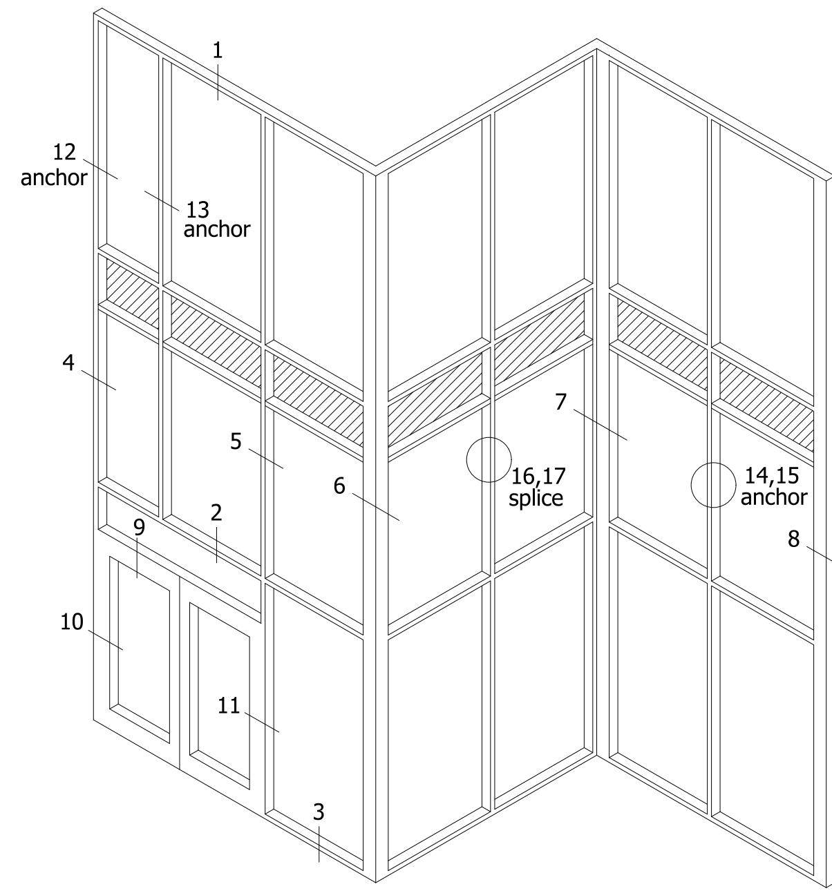
TYPICAL ELEVATION
