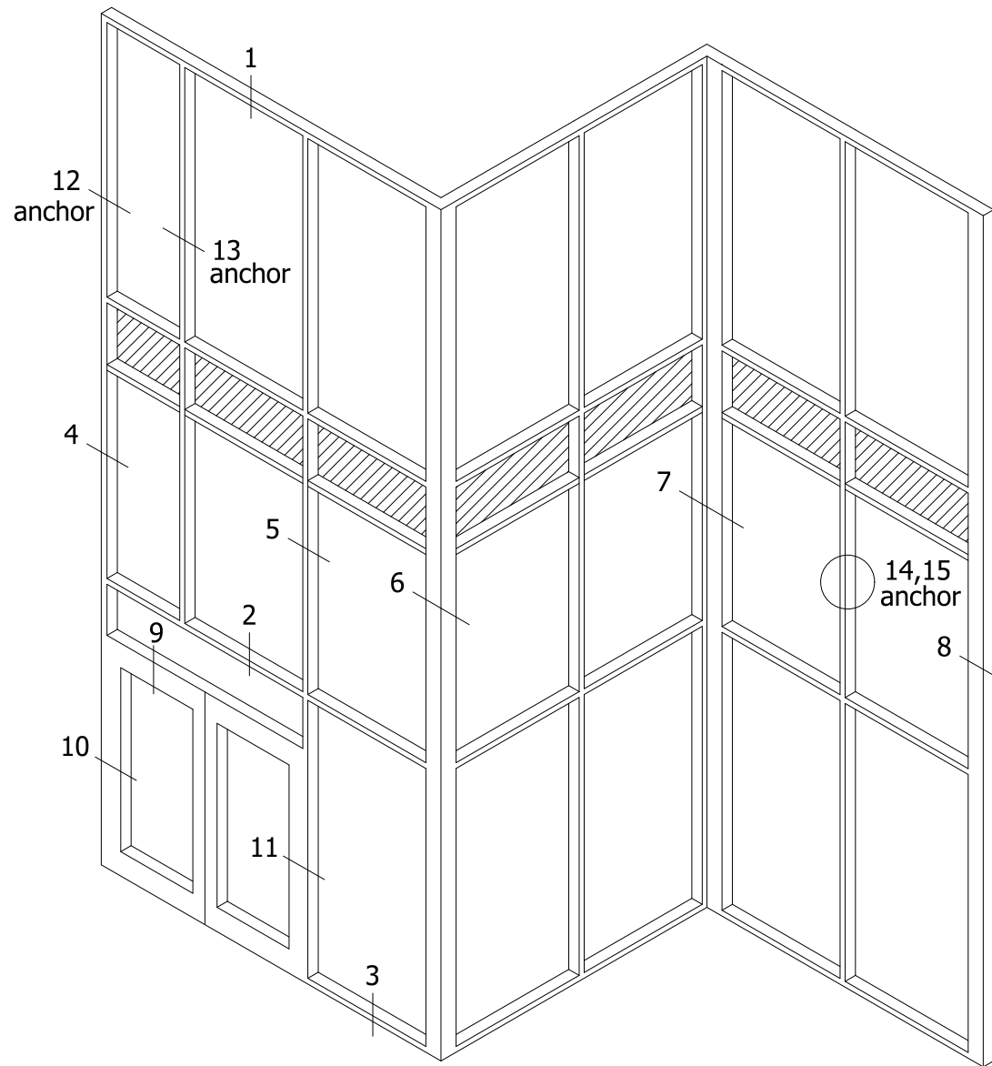
TYPICAL ELEVATION
