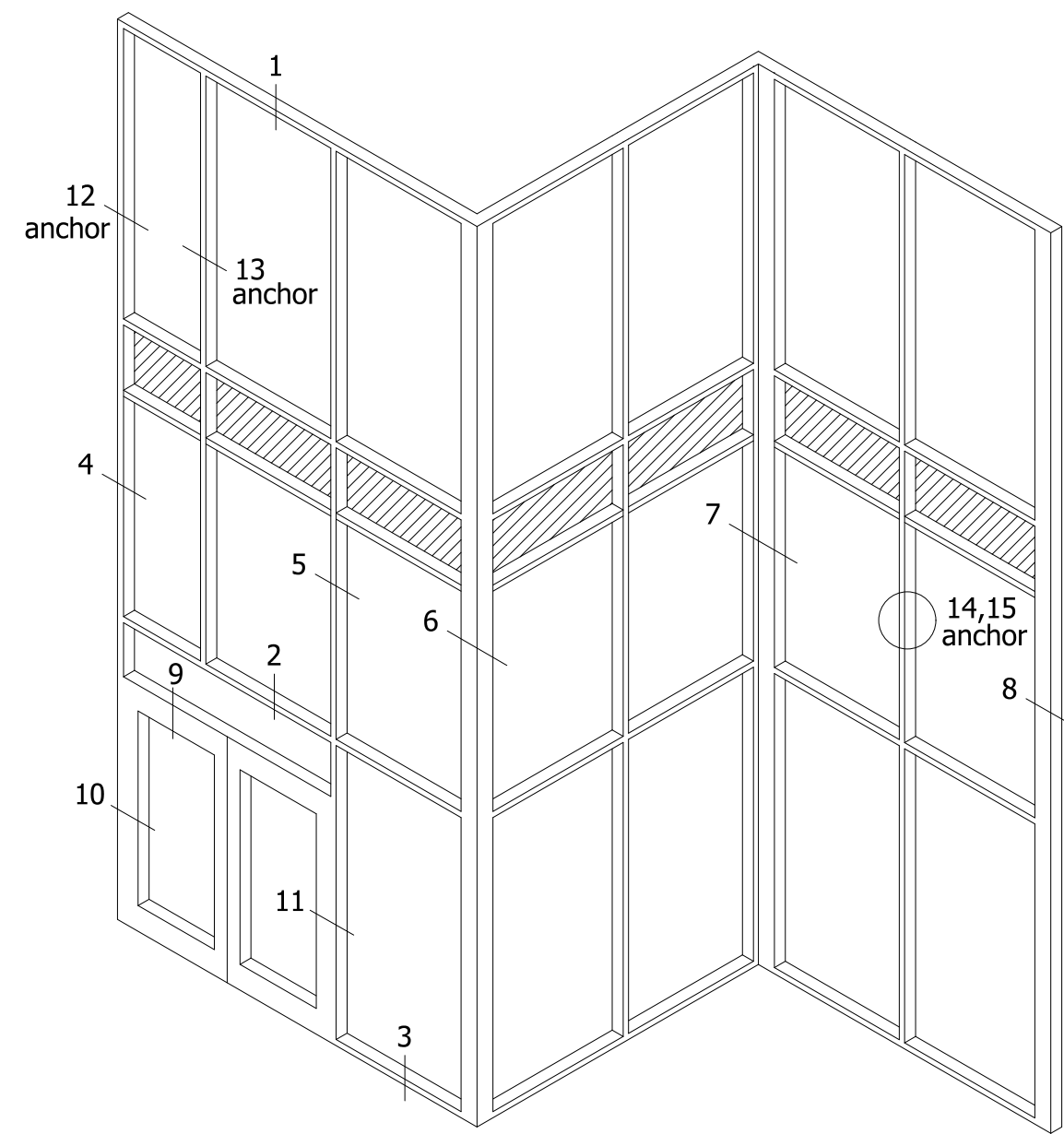
TYPICAL ELEVATION
