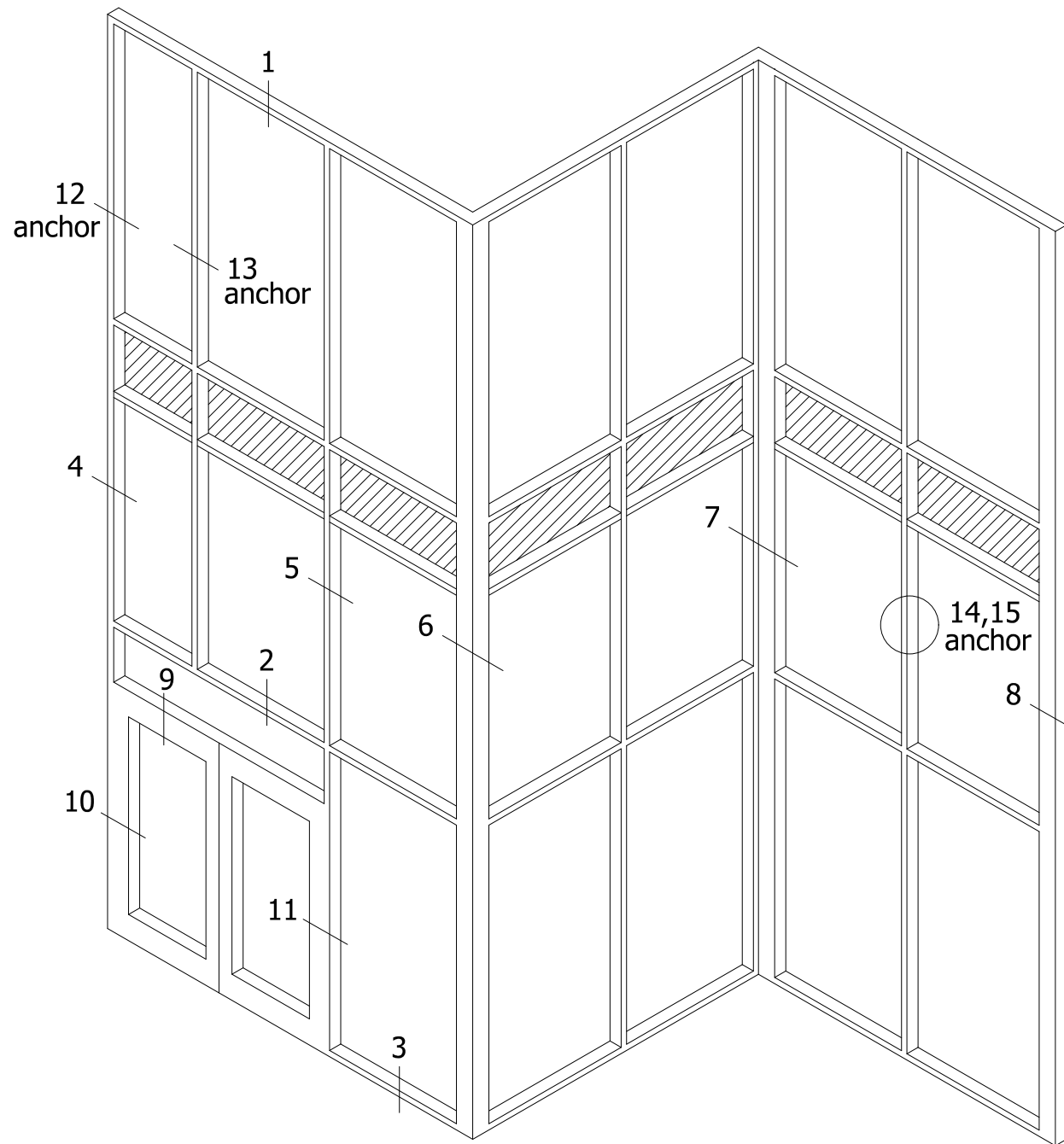
TYPICAL ELEVATION
