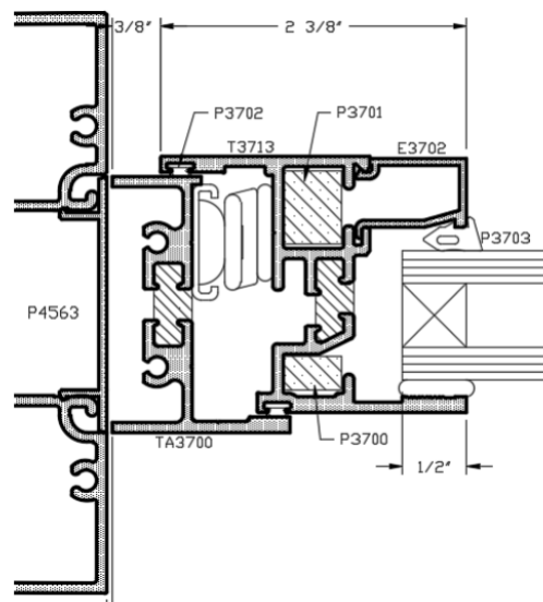
HW3700 Hopper Insert Vent (project-in)
